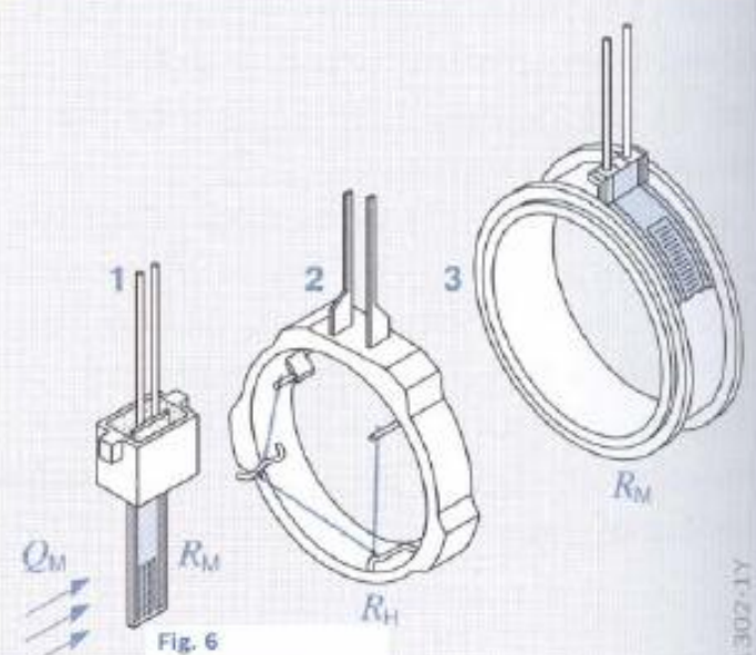
Fig. 6 1 Temperature compensation resistor R_K 2 Sensor ring with hot wire R_H 3 Precision measuring resistor ( R_M ) Q_M Air-mass flow
