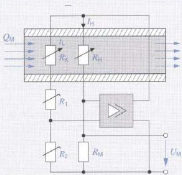
Fig. 5 Q_{M,0} Air-mass flow U_M Measurement voltage R_H Hot-wire resistor R_K Compensation resistor R_M Measuring resistor R_{L,0} Calibration resistors
