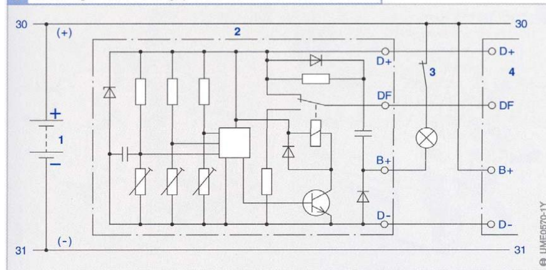
3 Circuit diagram of an overvoltage-protection device for a Double-T1 alternator
