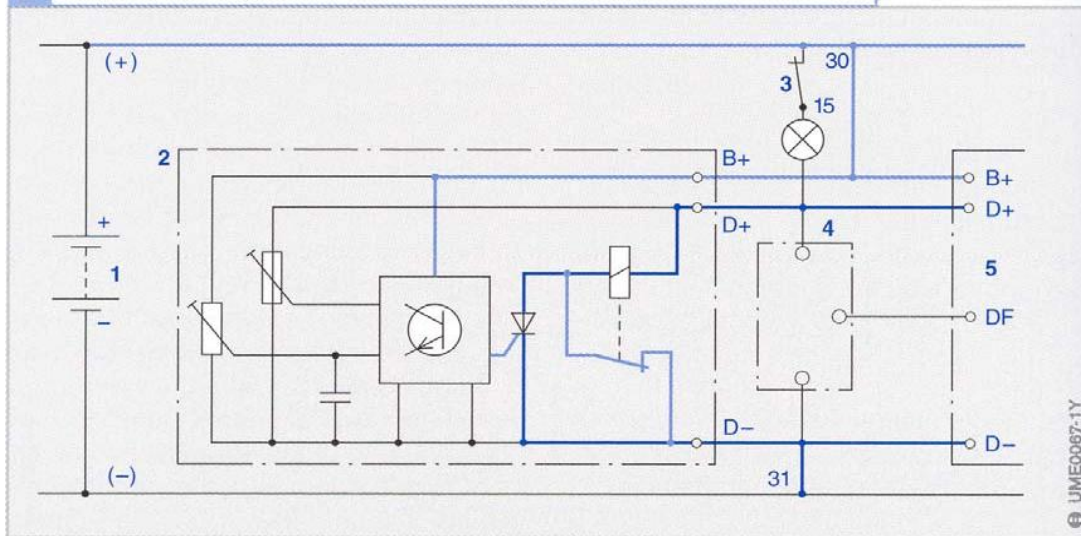
2 Simplified circuit diagram of an automatic overvoltage-protection device for a T1 alternator
