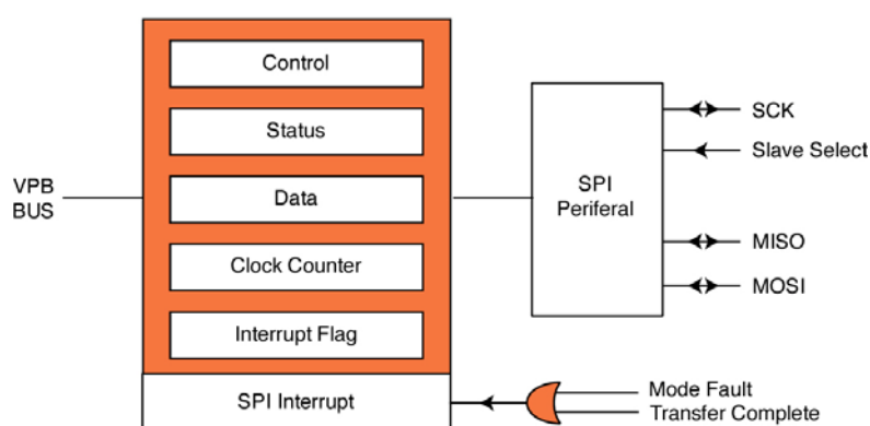
SPI Register Interface
