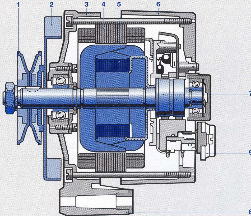
4 Claw-pole alternator with compact diode assembly: Section drawing
