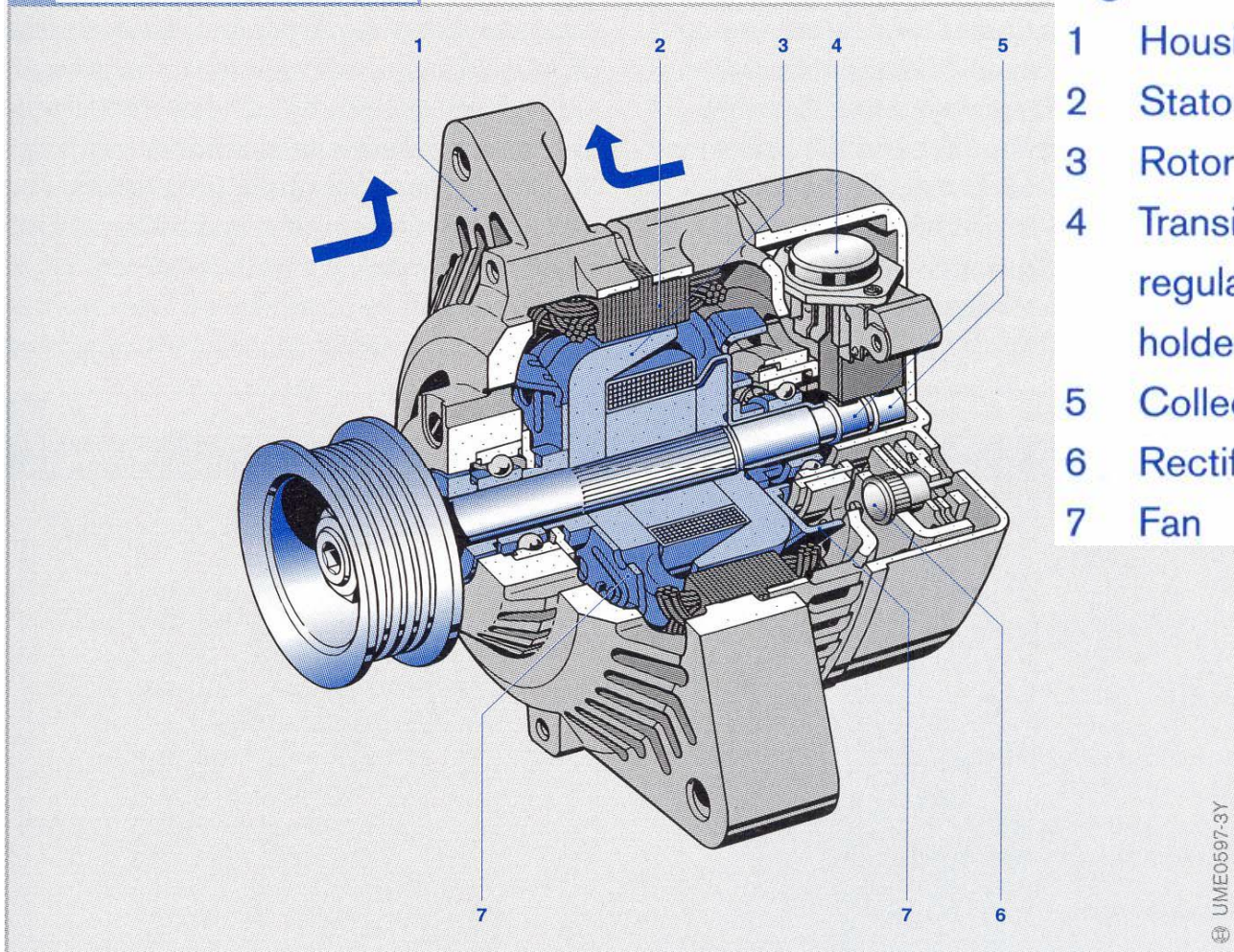
14 Design of the compact alternator
