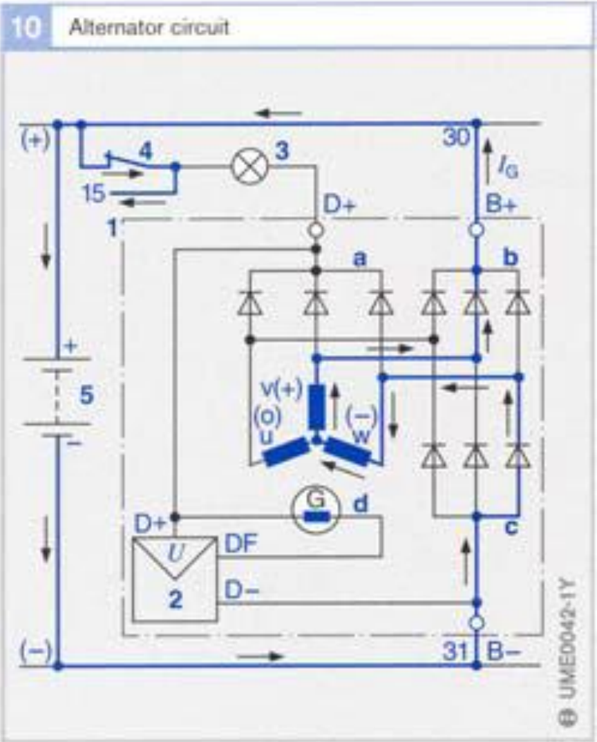
Fig. 10 1 Alternator 1a Excitation diodes 1b Positive-plate diodes 1c Negative-plate diodes 1d Excitation winding 2 Voltage regulator 3 Charge-indicator lamp 4 Ignition switch 5 Battery
